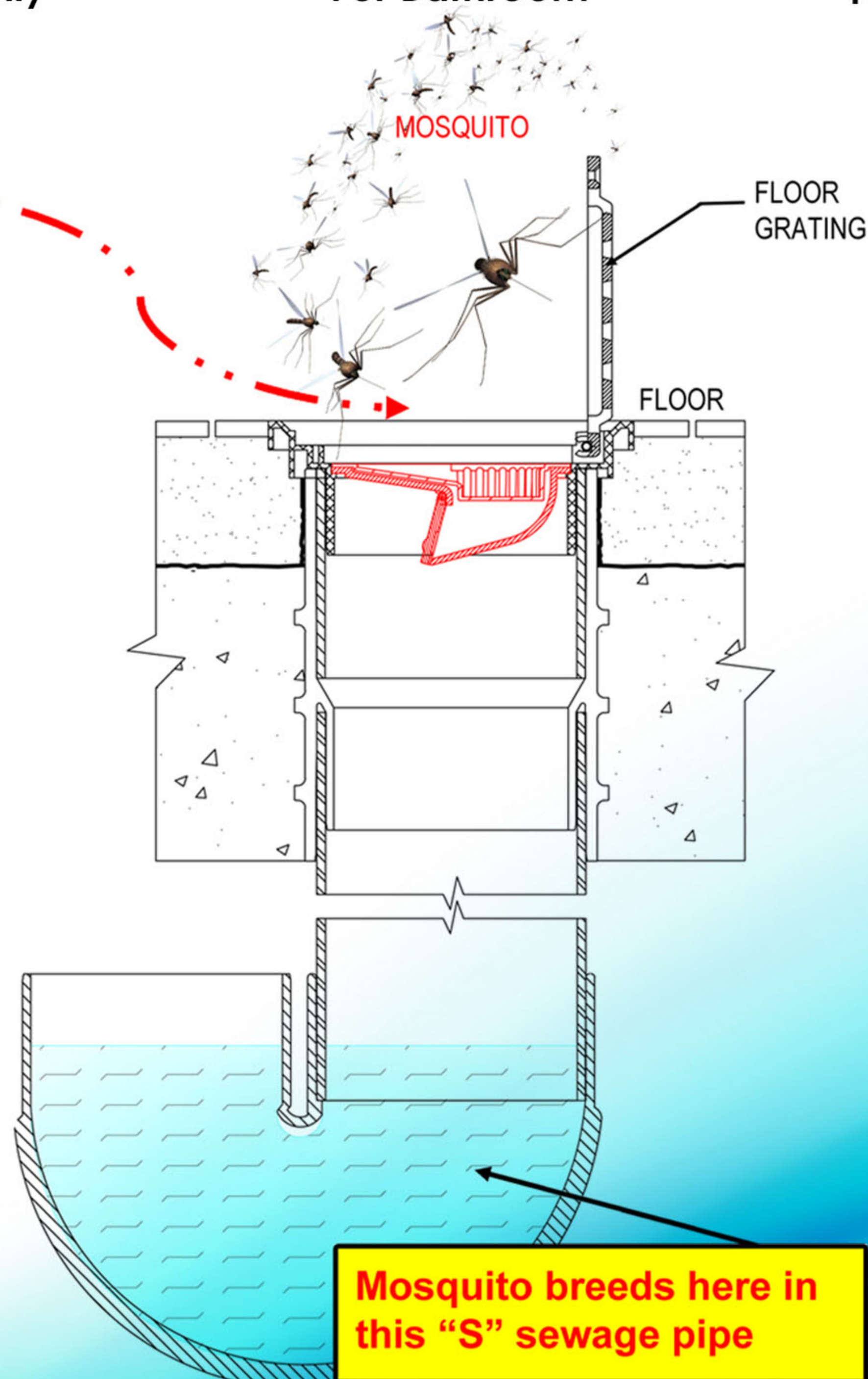
AMD98S Anti-Mosquito Device (Short) * For Bathroom
