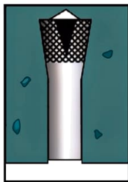
(4) Anchor is expanded
