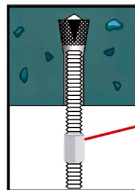
(5) Anchor is set with fastening bolt
