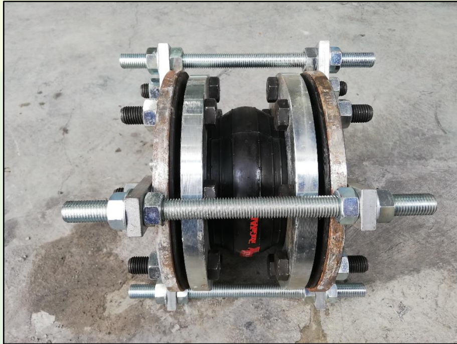
Figure 2: Photograph of 6" Single Bellow c/w.
