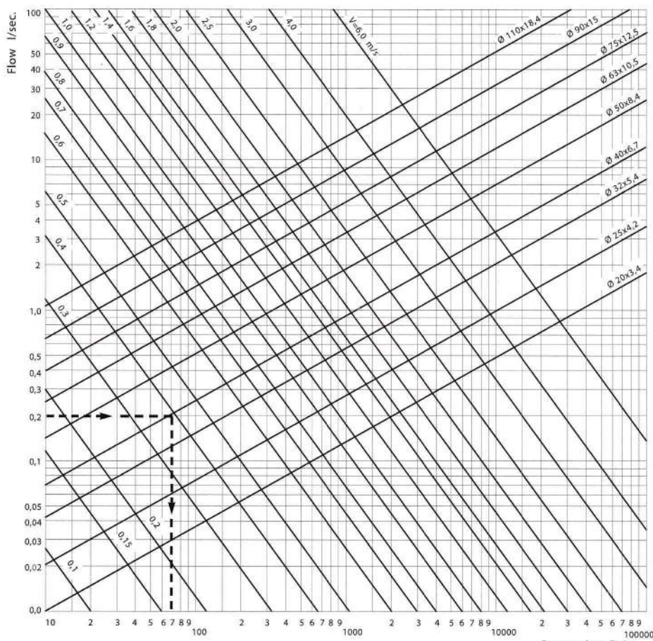
Loss Pressure Diagram for PN 20 Pipe
